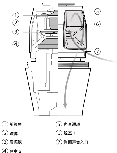
Dualdyne 话筒头侧视图
